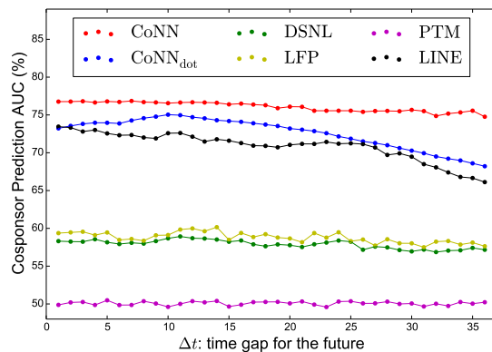
Figure 11: AUC score for cosponsor prediction.
