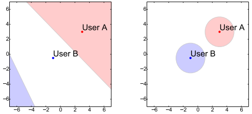
(a) Inner product-based similarity (b) Distance-based similarity
