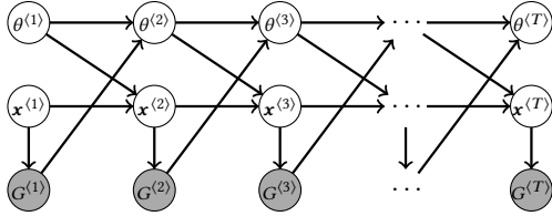
Figure 8: Graphical model representation of our model. Shaded units represent observed variables.
