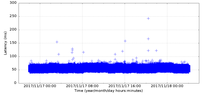
Fig. 8. Update latencies over 30-hour wide-area deployment
