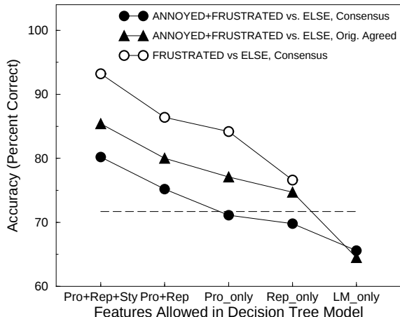
Fig. 1. Comparison of annoyance and frustration detection with different input features. Pro = prosody, Sty = Style, Rep = repetition/correction feature. The dashed line indicates accuracy for human interlabeler agreement on the first task.
