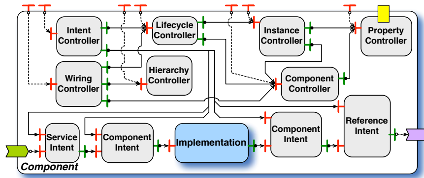
Figure 4. Personality Level.
