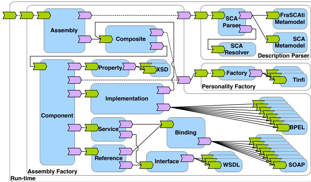
Figure 5. Run-time Level.
