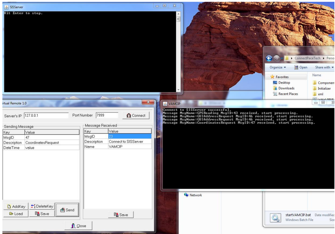
Figure 6 Message #47
