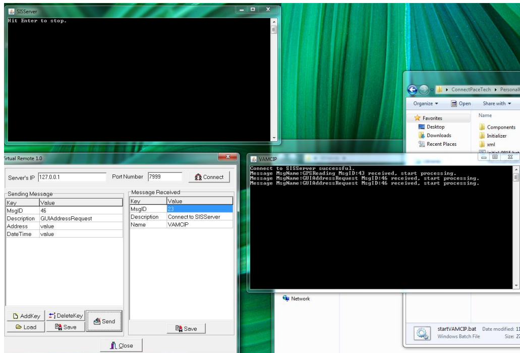
Figure 5 Message #46
