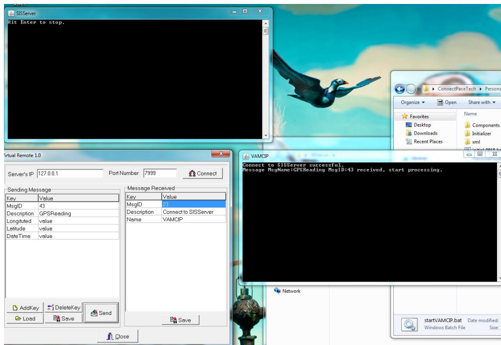
Figure 4 Message #43
