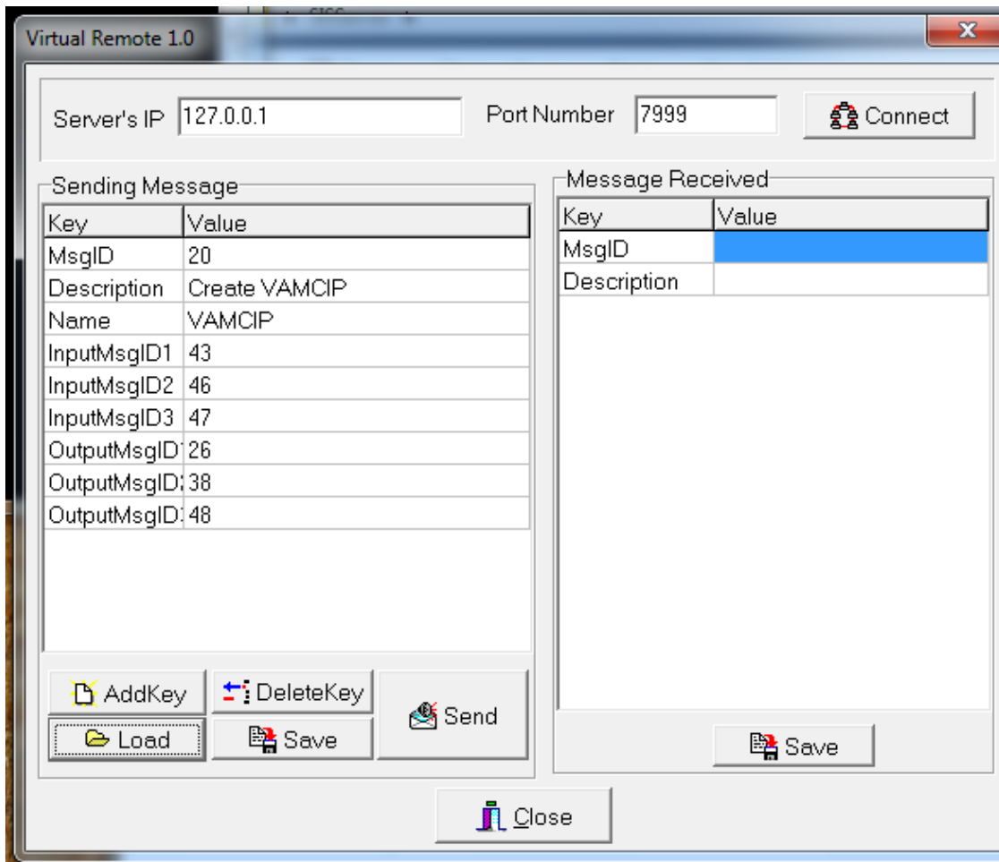
Figure 2 prjRemote Application
