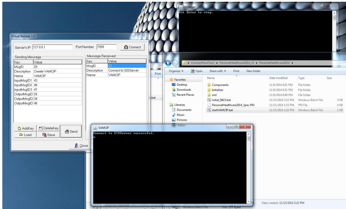
Figure 3 Control Messages
