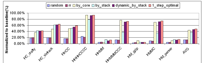
Fig. 11. Thermal emergency time reductions in heterogeneous floorplans.
