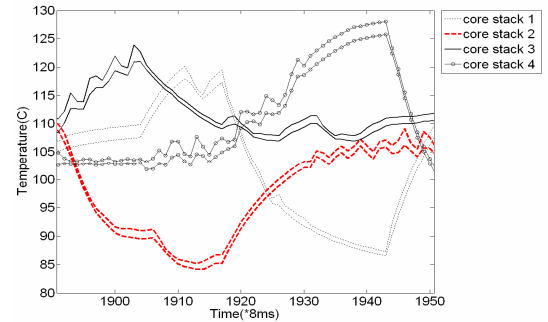
Fig. 3. Thermal correlation between adjacent dies.
