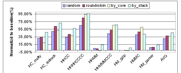
Fig. 9. Thermal emergency time reductions in homogeneous floorplans.
