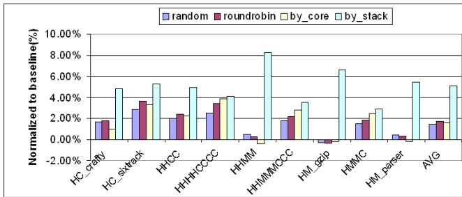
Fig. 10. Performance speedups for homogeneous floorplans.
