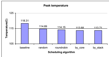
Fig. 8. Peak temperatures of different scheduling algorithms.
