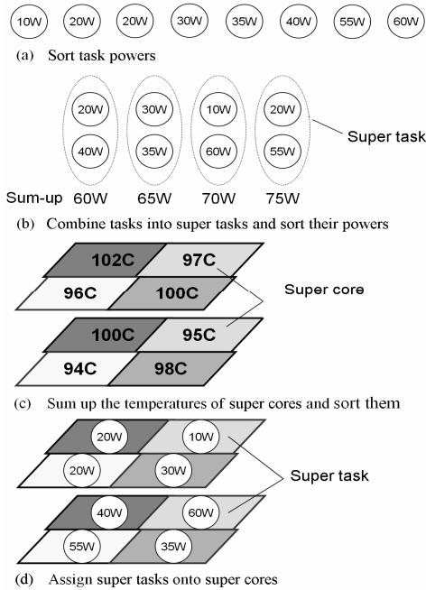
Fig. 5. The temperature balancing-by-stack algorithm.
