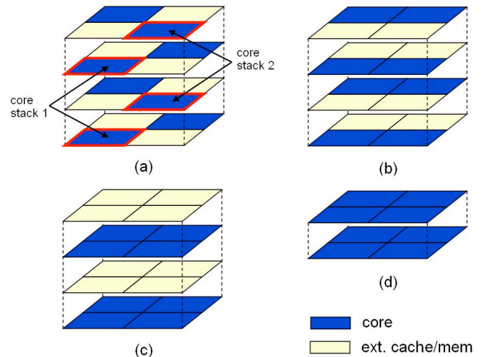
Fig. 1. 3D chip multiprocessor floorplan options.
