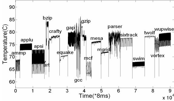
Fig. 6. Temperatures of the benchmark in SPEC2000
