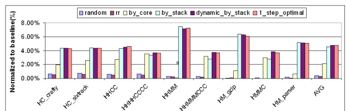
Fig. 12. Performance speedups for heterogeneous floorplan.
